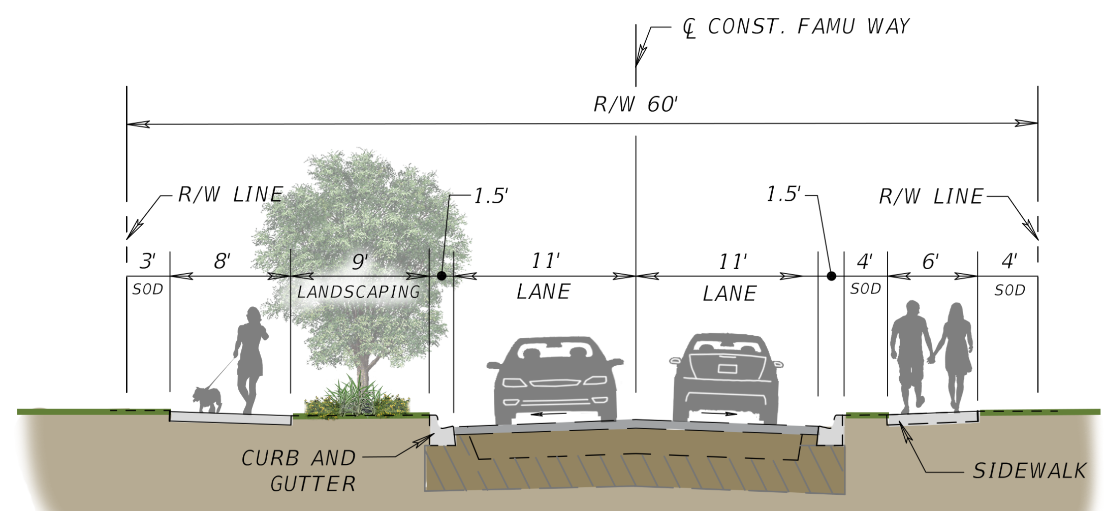
SECTION B-B'
